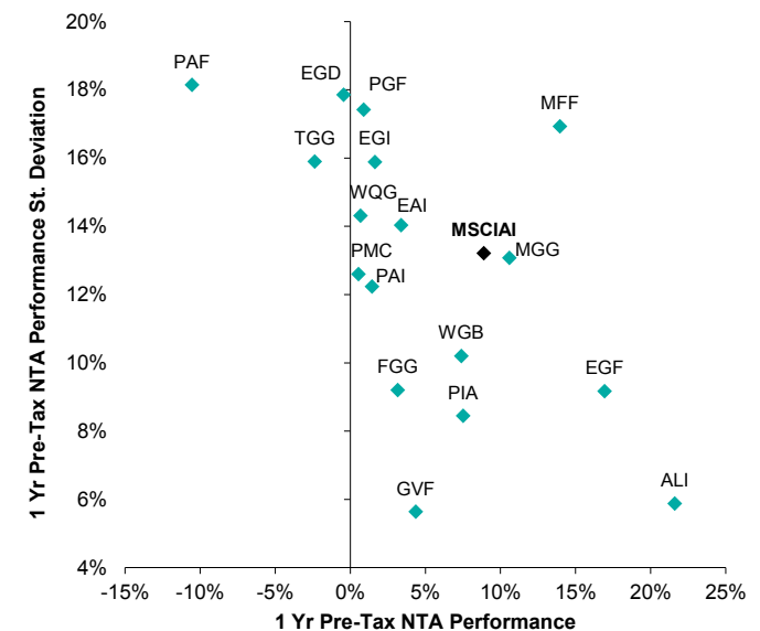
Figure 19 - 1yr Pre-Tax NTA Performance v Standard Dev.
